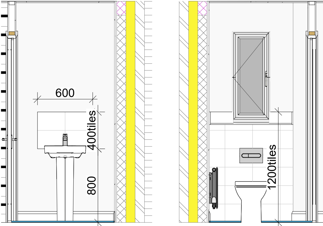
A WC - View A 1 : 25
