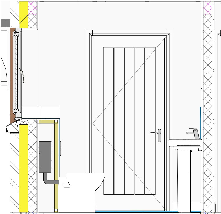
C WC - View C 1 : 25
